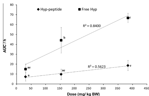
Fig. 3. Relationship between the Hyp area under the curve (AUC)/h and collagen hydrolysate dose. The AUC/h of free Hyp ( \blacksquare ) and peptide-bound Hyp ( \blacklozenge ) were calculated by the linear trapezoidal method from the data of 4 subjects after ingestion of collagen hydrolysate (30.8, 153.8 and 384.6 mg/kg body weight [BW]). Data are shown as the mean \pm SD; n = 4 . Different letters adjacent to data points indicate significant differences ( P < 0.05 ).
